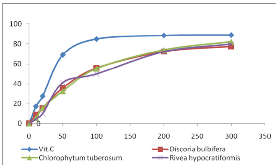
Figure 1. DPPH scavenging activity.
