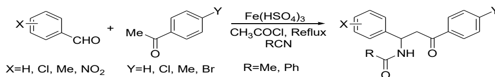
Scheme 3: Synthesis of \beta -amido ketones and esters
