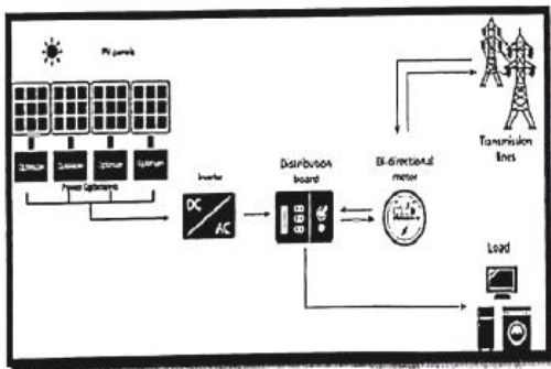
Photo 5 & 6: Conceptual Diagram: PV Grid Tied Solar System & field visit
