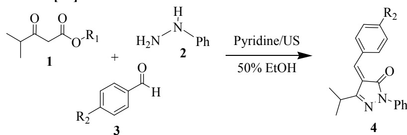
Figure I: Synthesis of 4-aryl methylenepyrazol-5(4 H )-ones
